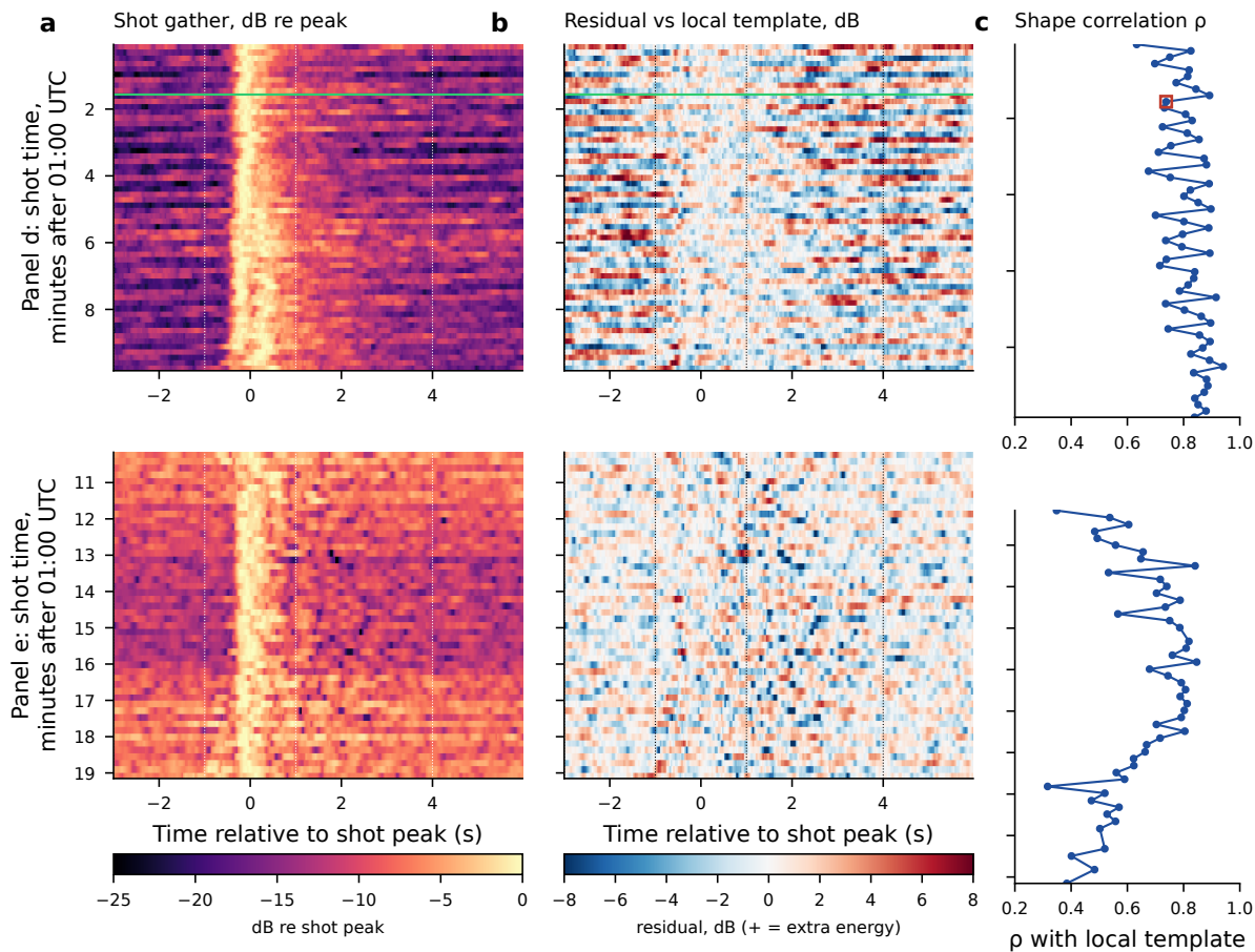
Each row is one H085 airgun-like shot (110 shots, 9.95 s cadence; weak secondary pulses excluded), from Kadri (2024) Fig. 9 vectors (01:00–01:20 UTC 8 Mar 2014; filtered 2–40 Hz, single channel, vertex-simplified). Rows show the 0.25 s energy envelope, aligned by cross-correlation ( \pm 0.5 s). (a) envelope relative to each shot's peak (median of the \pm 6 neighbouring shots, levelled on the peak window, so the residual is zero there by construction); dotted lines mark the pre (–3 to –1 s), peak, post (1–4 s) and tail windows. (c) shape correlation with the local template, median 0.79; red square / green line = the single PCA outlier (01:01:33.8, H01W coincidences at chance). No shape or shoulder residual exceeds 3 robust \sigma . Injection: 50 % detection at –3 dB relative to a median shot. Pre-registered h085_shot_template.py (360bf14). No impact-PDF input in this figure.
